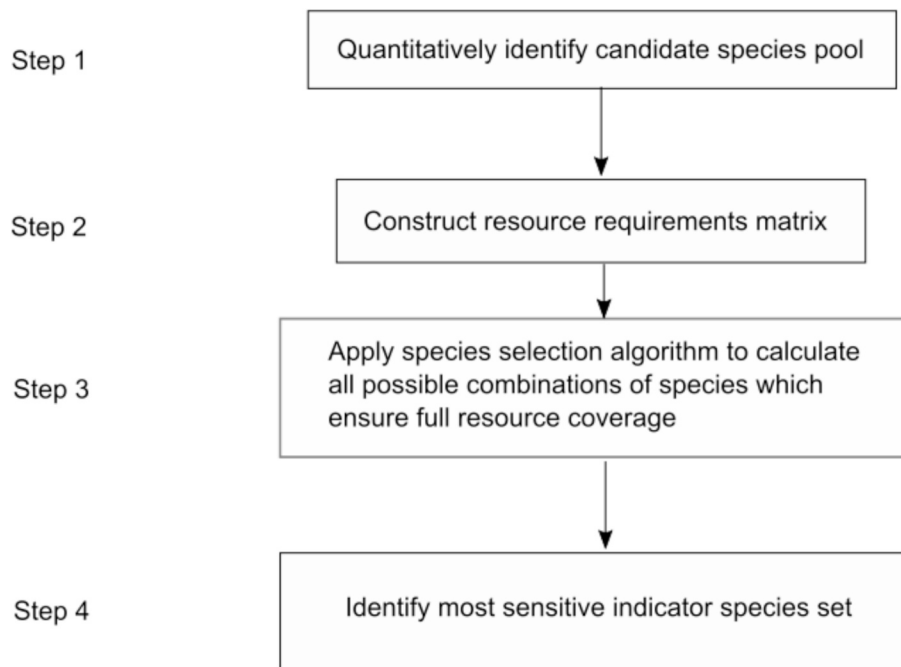
Fig. 1. Outline of the niche-based framework for indicator species selection (adapted from Butler et al., 2012). Each indicator set produced by the species selection algorithm in Step 3 receives an average sensitivity score which is the average sensitivity score across its constituent species. Each species' sensitivity score is calculated as the percentage of resources used divided by its reliance on forest habitat at the appropriate spatial scale. Detailed description of key processes and, where appropriate, quantitative thresholds or requirements to be met in each step of the niche-based framework are outlined in Table A.5.
