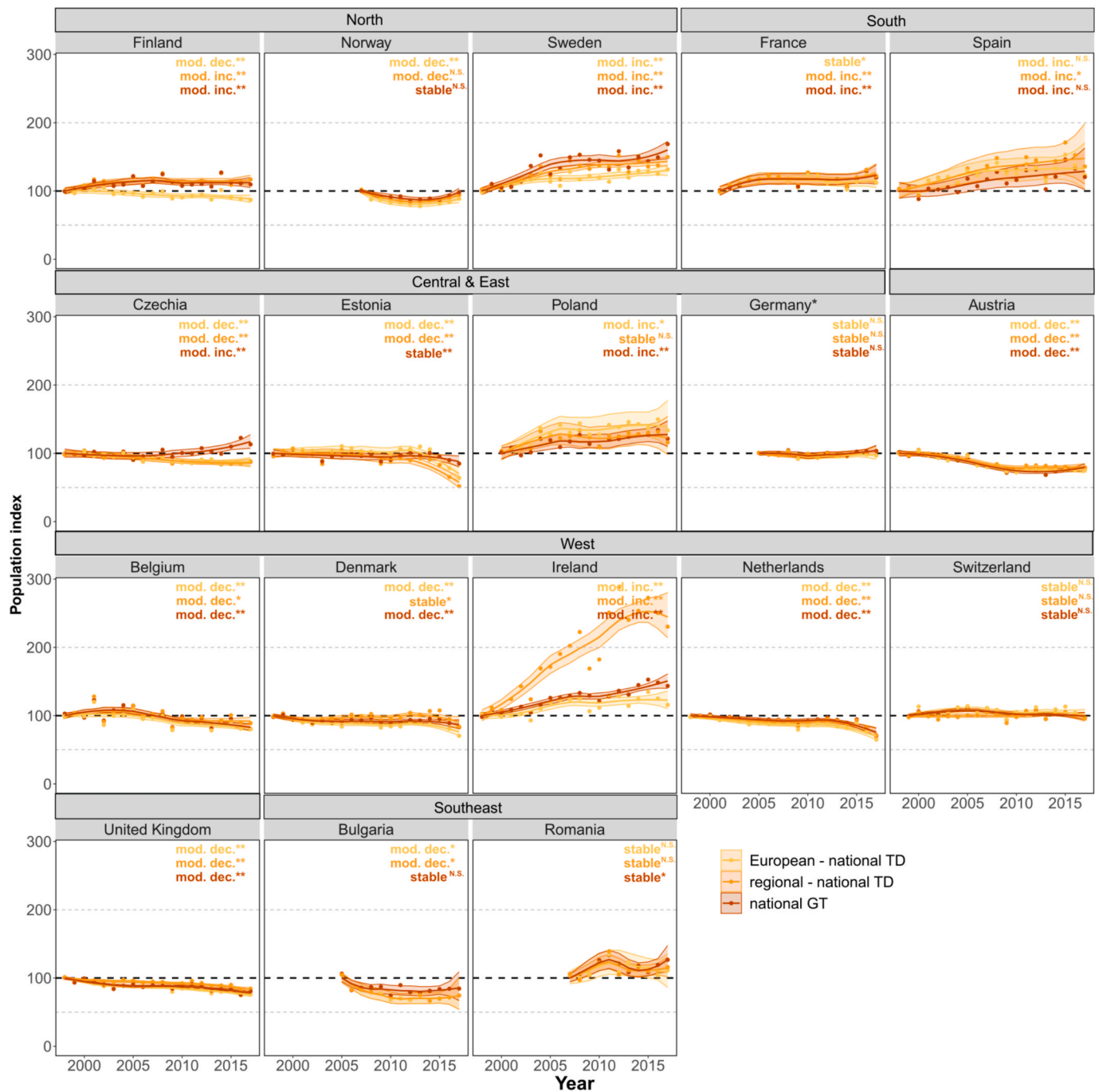
Fig. 6. Smoothed multi-species indices (MSIs), with shaded 95 % confidence intervals, for national GT , European – national TD , and regional – national TD indicator sets. The regional – national TD indicator set for Germany was derived from the aggregated indicator sets for the Central & East and West regions. The indicators for Belgium only represent the south (Wallonia) as data were not available for northern Belgium. Indices were set to 100 and their SEs to 0 in the first year where data were available for each given country. Description of the overall trend for each index, and significance of those trends, are provided in the upper right corner; * = p < 0.05 , ** = p < 0.01 , N.S. = not significant. Note: national trends may differ from existing published national FoBIs produced by the countries themselves due to differences in indicator species selection methods employed.
