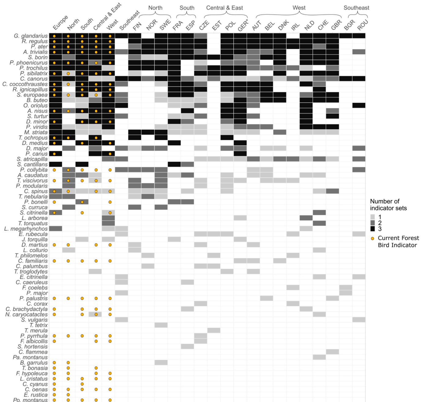
Fig. 2. Frequency of each species occurrence across indicator sets for Europe, for each region and each country. Countries are given a three-letter code (Table A.6) with species full names provided in Table A.7. Species can occur in a maximum of three indicator sets at each spatial scale (“geographically-targeted”, “top-down” from European set, “top-down” from regional set for national indicators; “geographically-targeted”, “top-down” from European set, “bottom-up” from national sets for regional indicators; “geographically-targeted”, “bottom-up” from regional sets, “bottom-up” from national sets for European indicators). For comparison, species that occur in the current European and four regional Forest Bird Indicators (FoBI) are also identified; no current regional FoBI for the Southeast region. *GER: regional – national TD indicator set is derived from both the Central & East and West regions of Germany. Equally, the national German indicator set contributes to both the Central & East and West national – regional BU indicator sets. The indicators for Belgium only represent the south (Wallonia) as data were not available for northern Belgium. Full details of species included in each indicator set for each spatial scale can be found in Appendix C.
