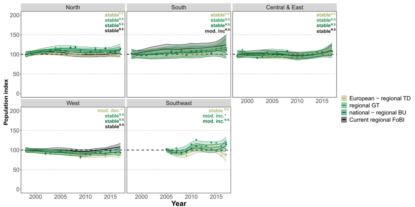
Fig. 5. Smoothed multi-species indices (MSIs), with shaded 95 % confidence intervals, for regional GT , European – regional TD , national – regional BU indicator sets and current regional Forest Bird Indicators (FoBIs) (where available). The national GT indicator set from Germany contributed to the national – regional BU indicator sets for both Central & East and West regions. Indices were set to 100 and their SEs to 0 in 1998 for North, South, Central & East and West, and in 2005 for Southeast. Description of the overall trend for each index, and significance of those trends, are provided in the upper right corner; * = p < 0.05 , N.S. = not significant.
