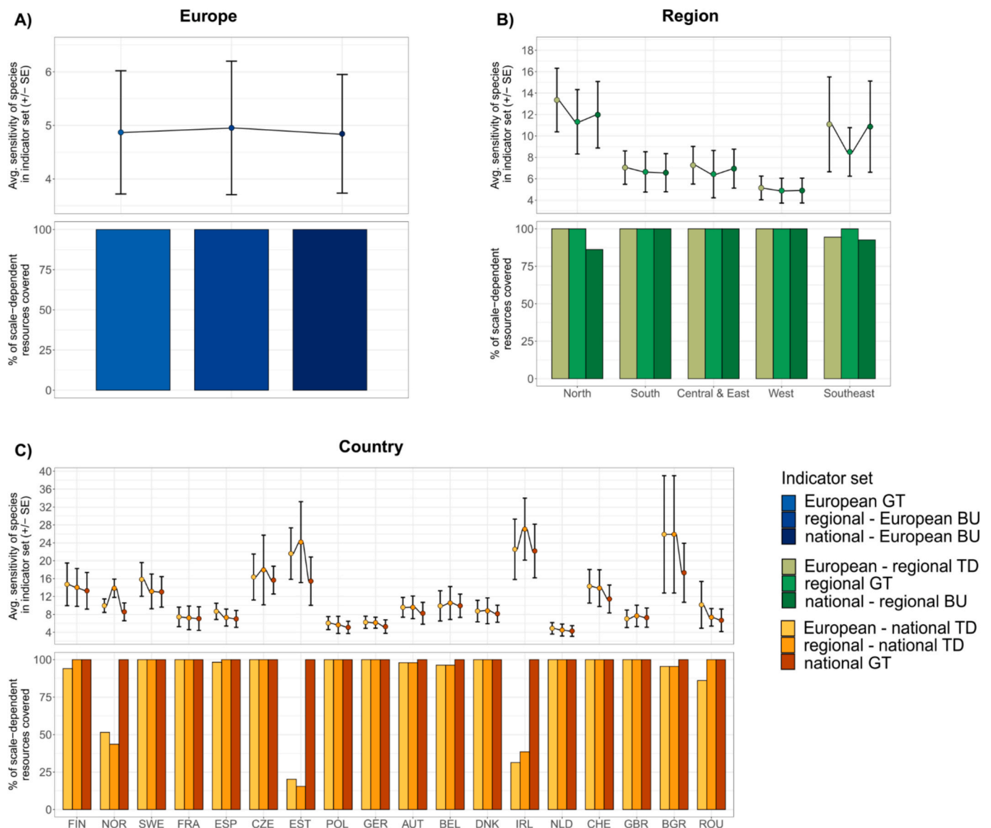
Fig. 3. Average sensitivity score ( \pm SE) (upper graph) and percentage of scale-dependent resources covered (lower graph) by, A) European, B) regional and C) national-level indicator sets. The indicator set type (“geographically-targeted”, GT; “top-down”, TD; “bottom-up”, BU) is provided alongside each indicator set. Each country is denoted by a three-letter code (Table A.6). Note that a higher score value indicates lower sensitivity.
