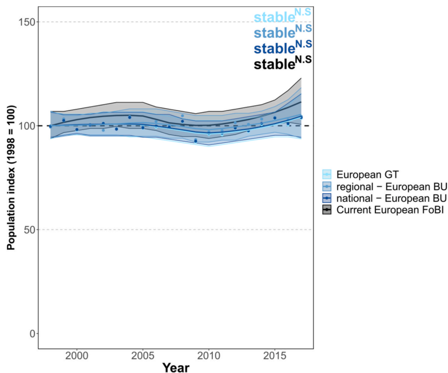
Fig. 4. Smoothed multi-species indices (MSIs), with shaded 95 % confidence intervals, for European GT , regional – European BU , national – European BU indicator sets and the current European Forest Bird Indicator (FoBI). Indices were set to 100 and their SEs to 0 in 1998. Description of the overall trend for each index, and significance of those trends, are provided in the upper right corner; N.S. = not significant.
